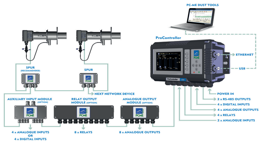
PCME QAL 360s sensors used in a network system
